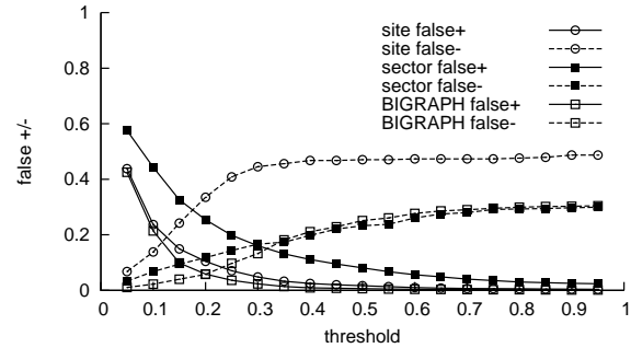
Figure 18: Anomaly detection via the re-assigned performance.
