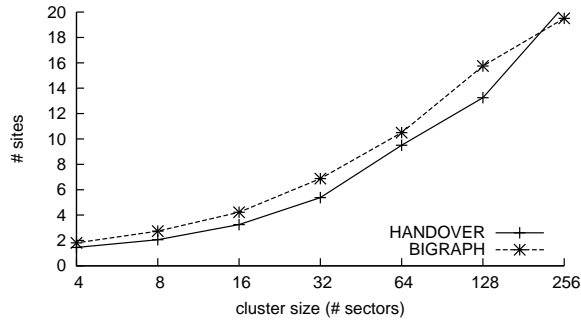
Figure 9: # cell sites covered by one BIGRAPH/HANDOVER cluster.
