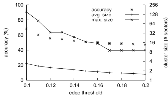
Figure 14: THRE's accuracy and average/maximum cluster size over threshold.
