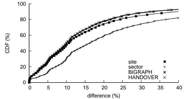
Figure 16: Difference across the re-assigned, measured, and ground truth performance.
