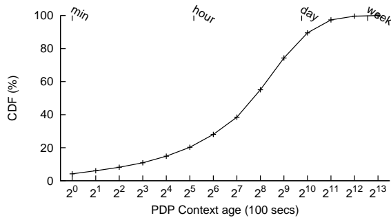
Figure 3: Age of PDP Context age of RNCGroundTruth records.
