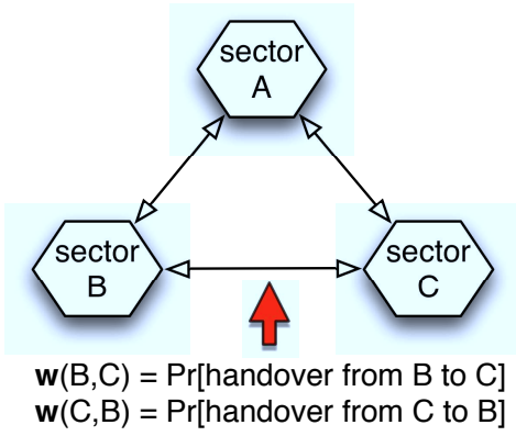
Figure 7: HANDOVER constructing the graph.
