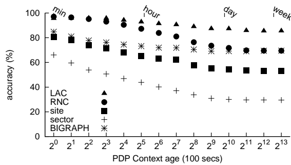
Figure 4: Accuracy over PDP Context age / BIGRAPH's accuracy over PDP Context age.
