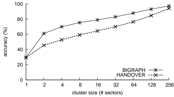
Figure 8: BIGRAPH’s and HANDOVER’s accuracy over cluster size.
