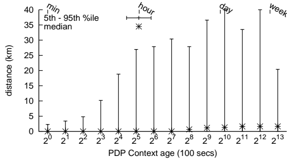
Figure 5: Distance from the site by PDPSetupLocations to the site by RNCGroundTruth.
