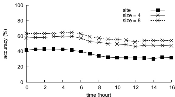
Figure 13: HANDOVER's accuracy over hours.
